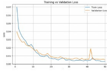
Figure 16: Training vs Validation for Hybrid sampling with cycling learning rate
