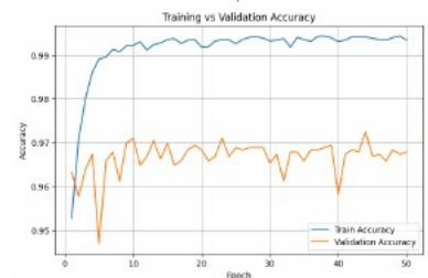
Figure 10: Training vs Validation Accuracy graph for Oversampling
